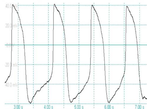
hIPS cardiomyocyte action potentials recorded with the Patchserver
